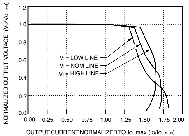
Figure 12. Lx010x/Lx015x Single-Output Normalized Output Current vs. Normalized Output Voltage at T_c = 25\text{ }^{\circ}\text{C}
