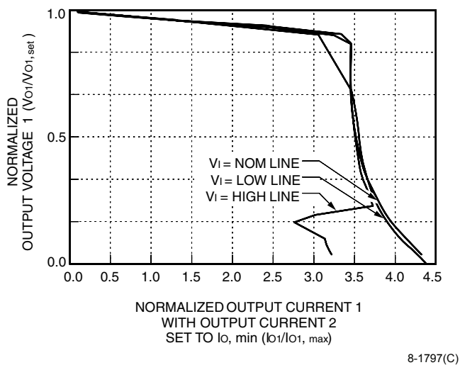
Figure 13. Lx010xx Dual-Output Normalized Output Current vs. Normalized Output Voltage at T_c = 25\text{ }^{\circ}\text{C} with Other Output at I_{o, \min}
