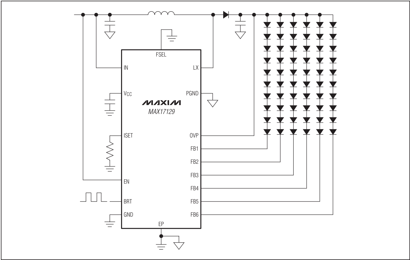
Simplified Operating Circuit
