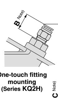
One-touch fitting mounting (Series KQ2H)
