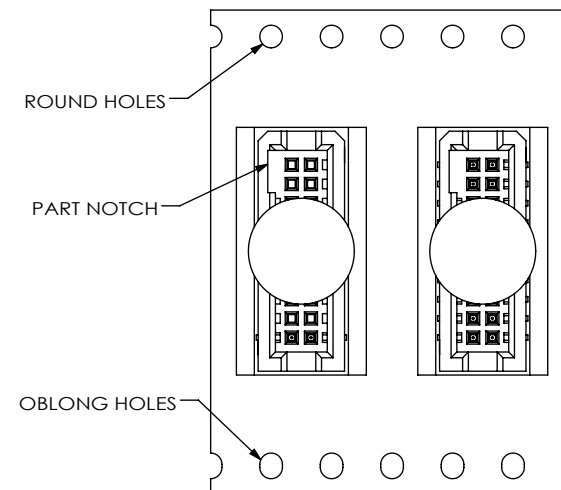
FIG 4 -TR: TAPE AND REEL
