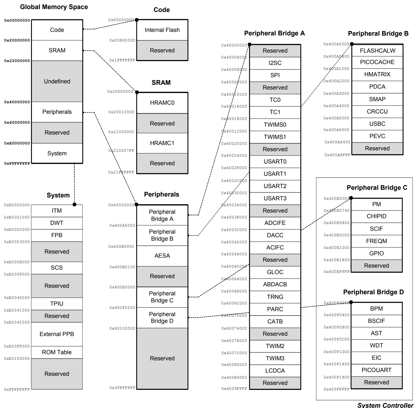
Figure 5-1. ATSAM4L8/L4/L2 Product Mapping
