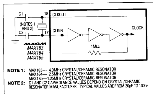
Figure 6. MAX183/184/185 Internal Clock Circuit
