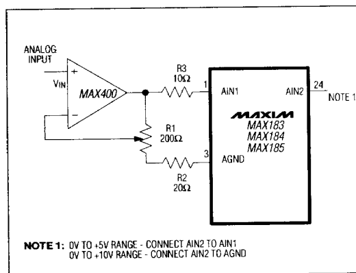
Figure 18. Unipolar Operation with Gain Adjust
