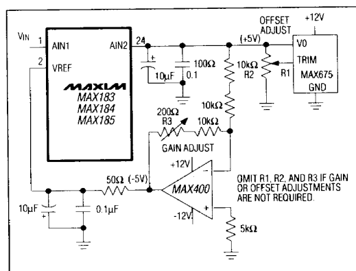
Figure 19. Bipolar Operation with Offset and Gain-Error Adjust
