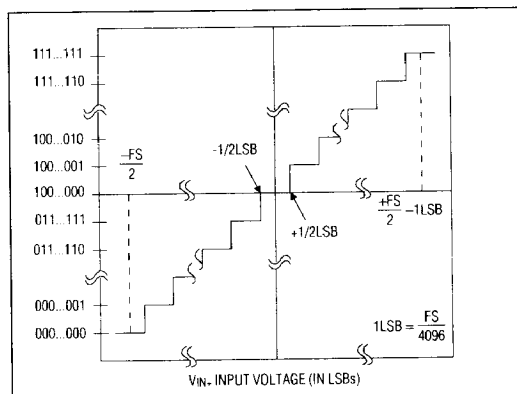
Figure 20. Ideal Input/Output Transfer Characteristic for Bipolar Operation
