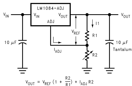
Figure 17. Basic Adjustable Regulator
