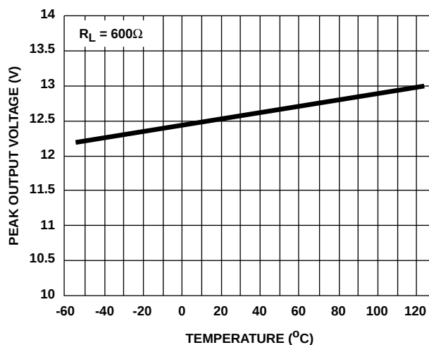
FIGURE 14. OUTPUT VOLTAGE SWING vs TEMPERATURE
