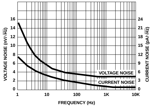
FIGURE 20. NOISE CHARACTERISTICS
