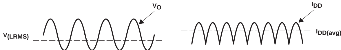
Figure 24. Voltage and Current Waveforms for BTL Amplifiers
