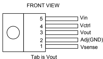
TO220-5L
