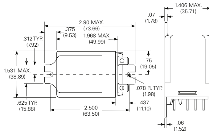
Bracket mount case
