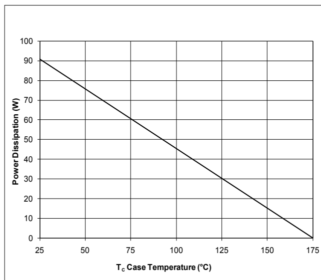
Figure 6. Power Derating
