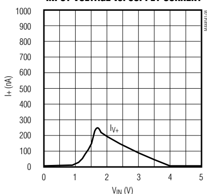
INPUT VOLTAGE vs. SUPPLY CURRENT
