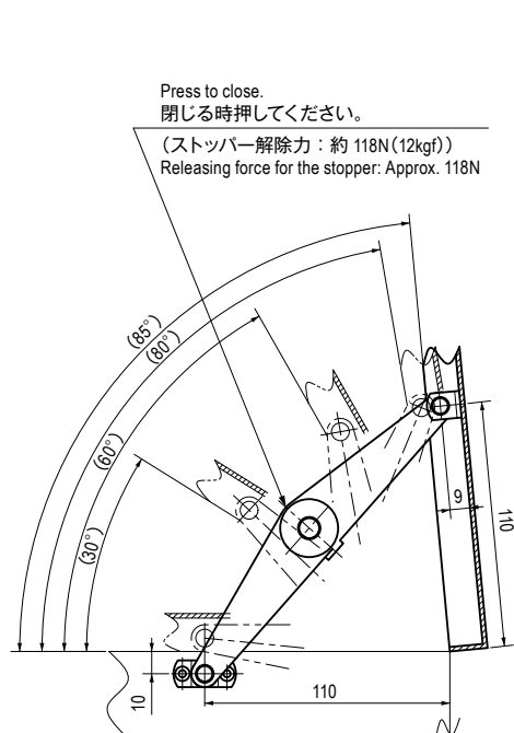
取付図 (蓋開閉角度) Installation Layout (Open and close angle of the lid)
