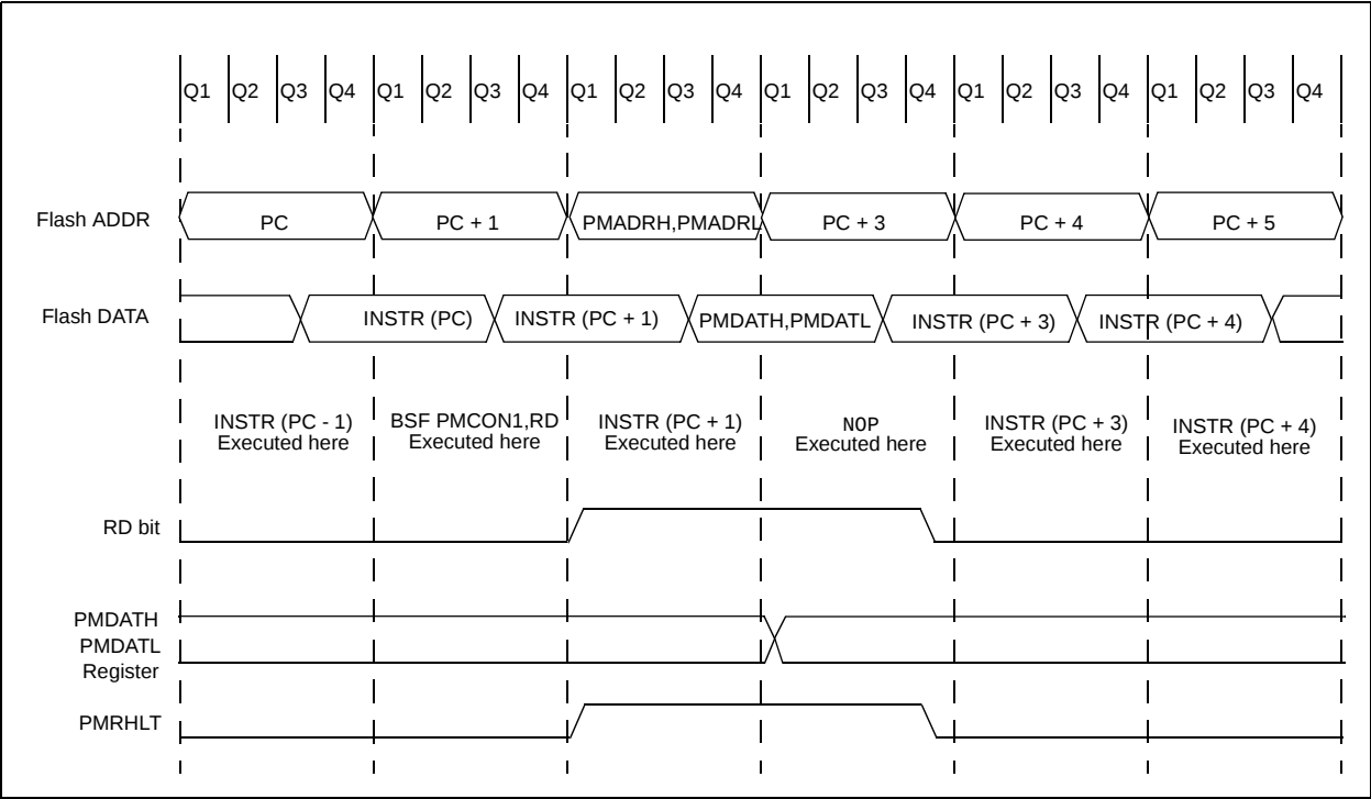
FIGURE 3-1: FLASH PROGRAM MEMORY READ CYCLE EXECUTION
