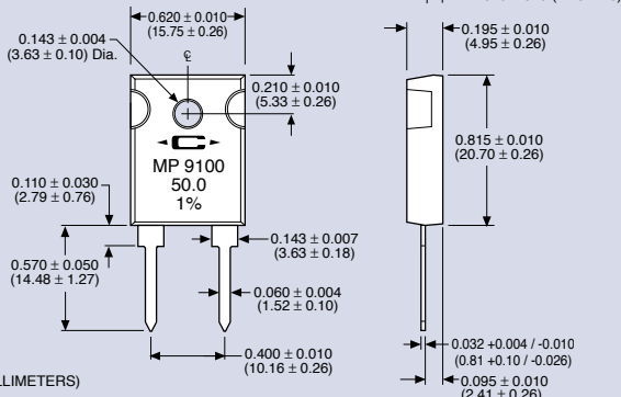
Figure 3 TO-247 Style MP9100
