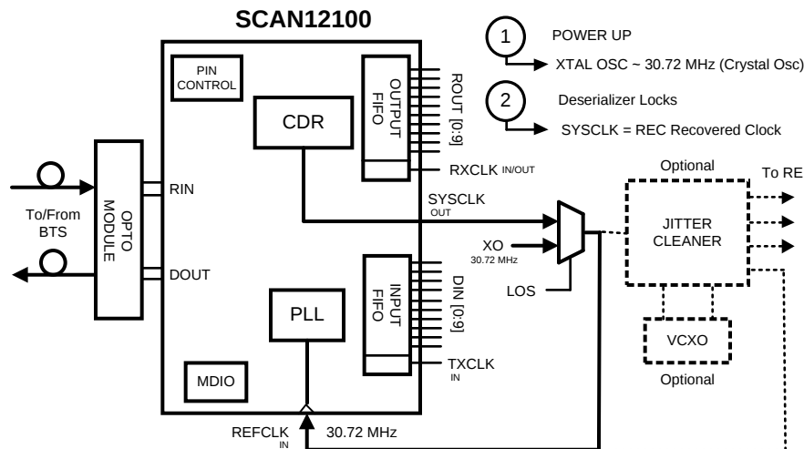
Figure 9. Radio Equipment (RE) Clock Synchronization
