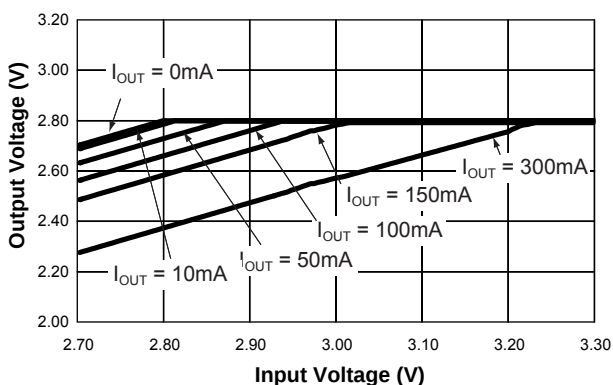
Dropout Characteristics
