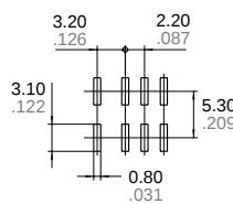
Suggested mounting pad
