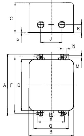
Housing L2
