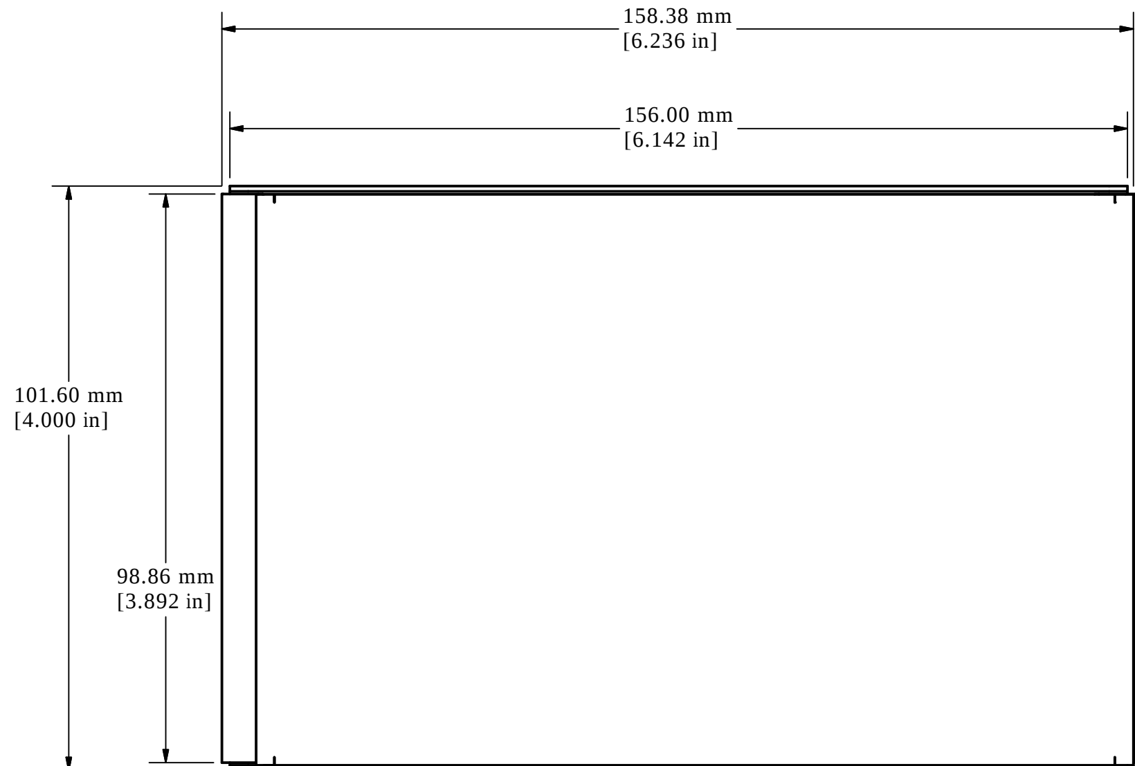
BOTTOM VIEW OF ASSEMBLY
