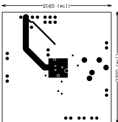
Figure 37. Recommended YZR PCB Layout: Mid Layer 2
