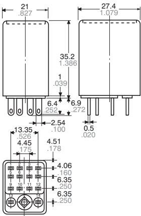
External dimensions
