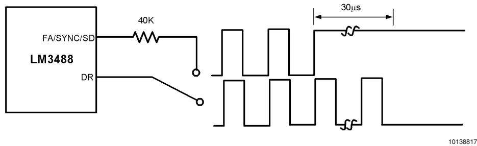
FIGURE 9. Shutdown Operation in Synchronization Mode
