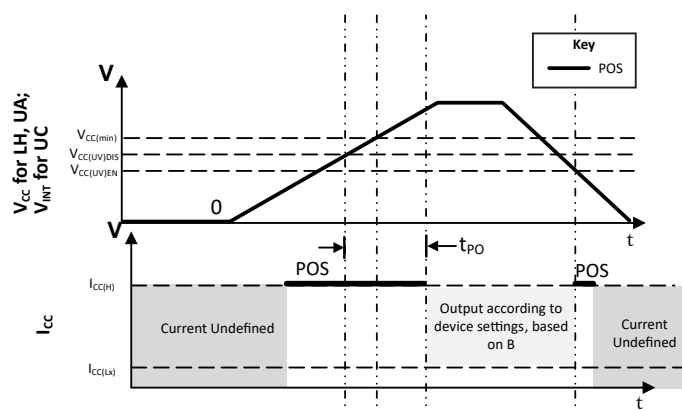
Figure 3: Power-On/UVLO Behavior
