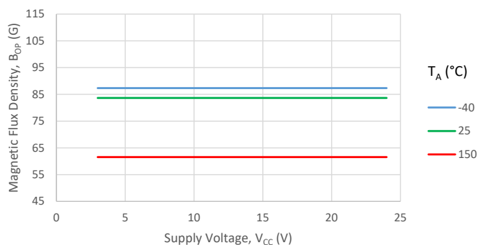
B_{OP(0)} vs. V_{CC}
