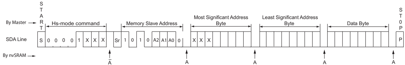
Figure 12. Single-Byte Write into nvSRAM (Hs-mode)
