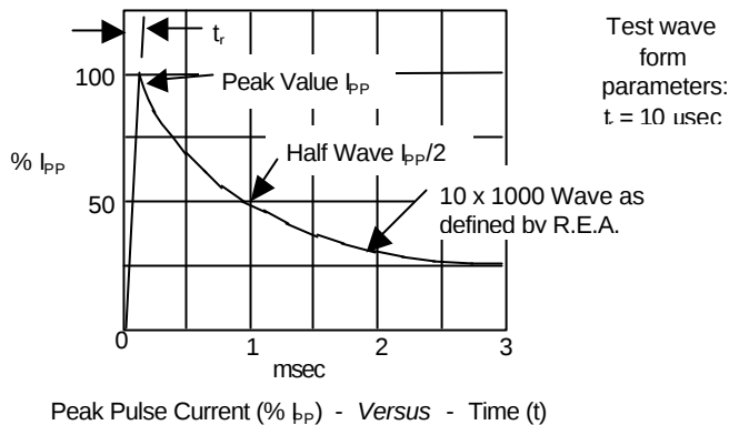
Figure 2 - Pulse Waveform
