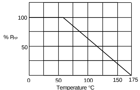
Figure 4 - Derating Curve
