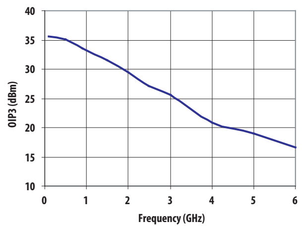
Figure 22. OIP3 vs Frequency at Id = 80 mA
