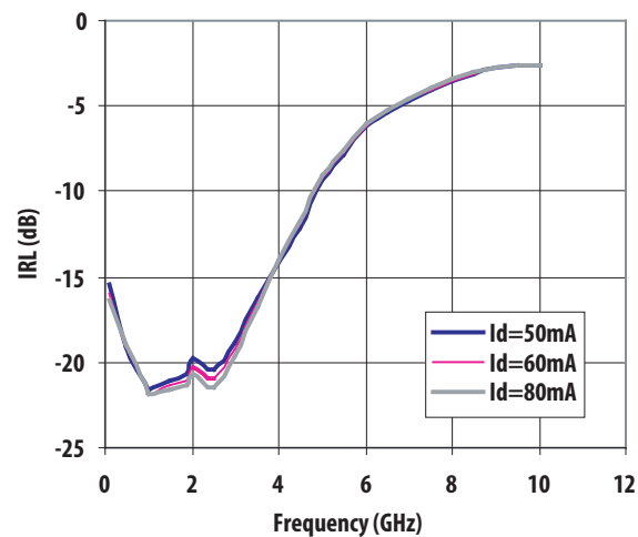
Figure 18. Input Return Loss vs Id and Frequency.
