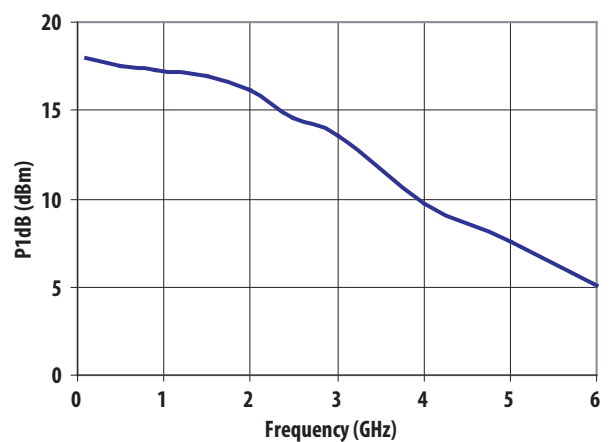
Figure 6. P1dB vs Frequency at I_d = 60\text{ mA} .
