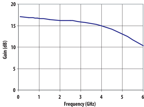
Figure 5. Gain vs Frequency at I_d = 60\text{ mA} .
