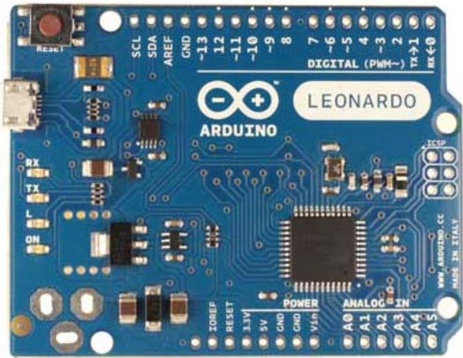
Arduino Leonardo Front without headers
