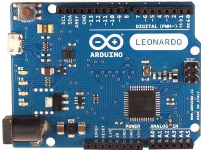
Arduino Leonardo Front with headers
