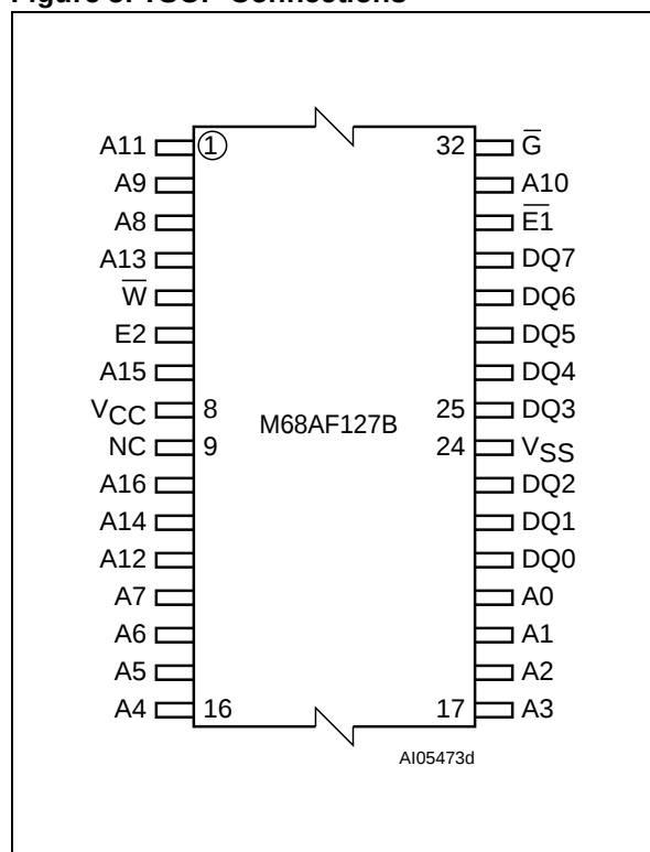
Figure 5. TSOP Connections
