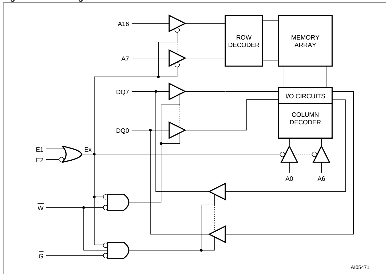
Figure 6. Block Diagram
