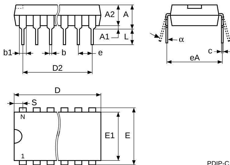
Figure 17. PDIP32 - 32 pin Plastic DIP, 600 mils width, Package Outline
