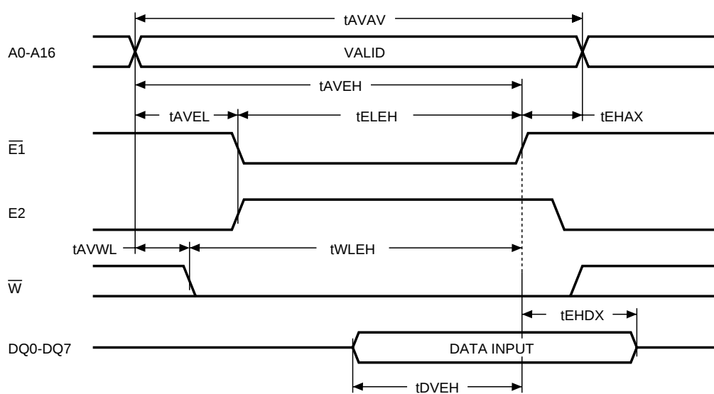
Figure 13. Chip Enable Controlled, Write AC Waveforms
