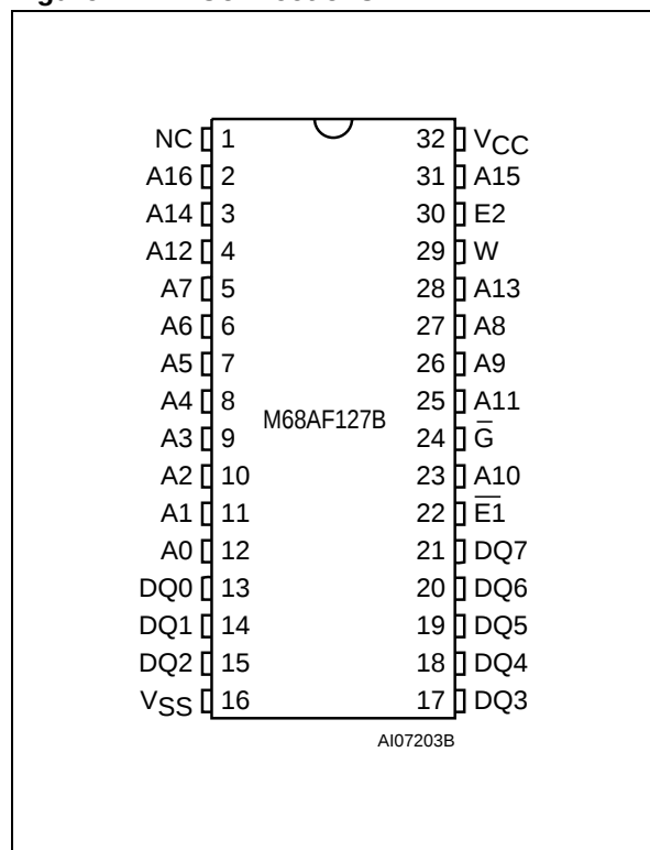
Figure 4. DIP Connections
