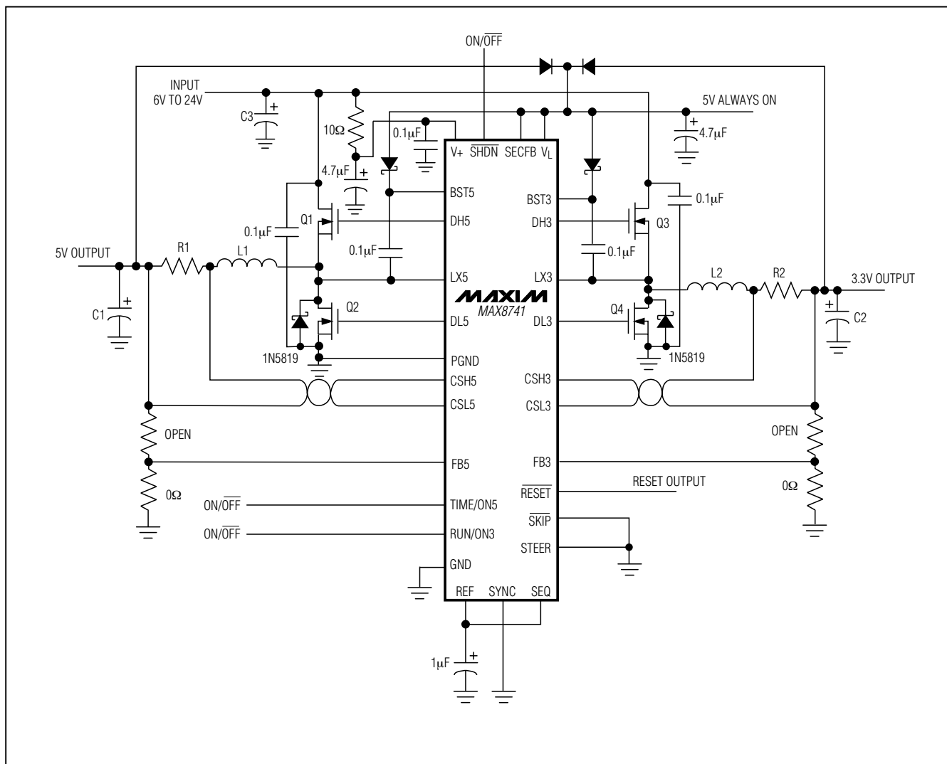
Figure 11. Dual 6A Notebook Computer Power Supply
