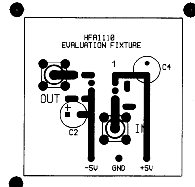
TOP LAYOUT
