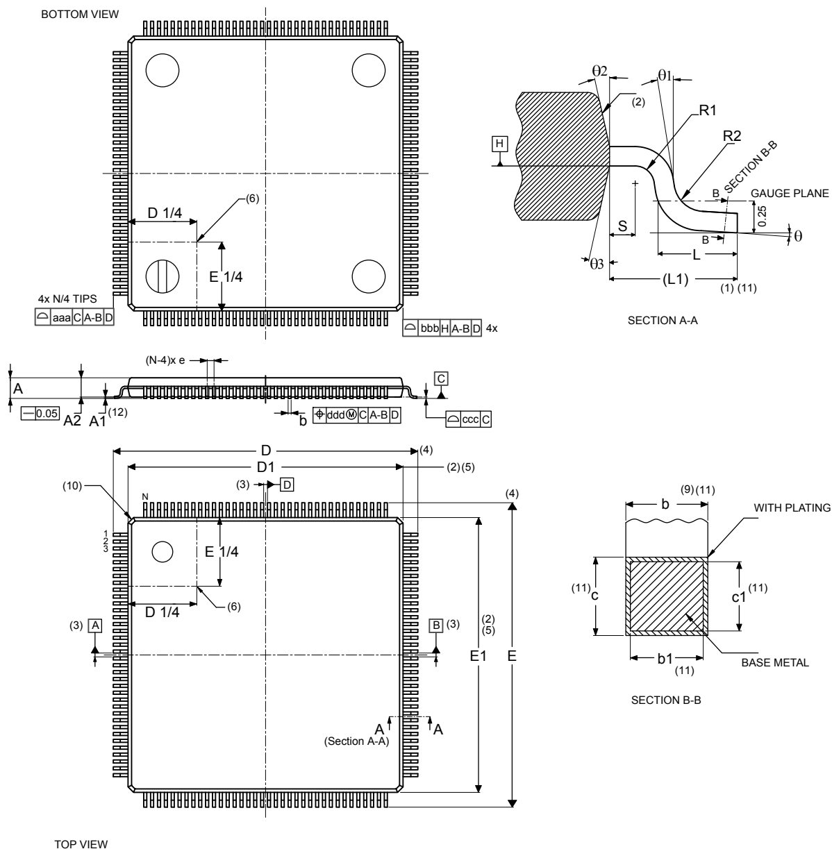
Figure 79. LQFP144 - Outline (15)
