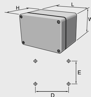
Montagemaß Mounting dimensions Montageafmetingen
