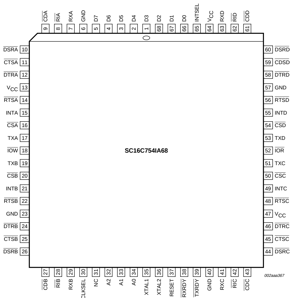
Fig 3. PLC68 pin configuration.
