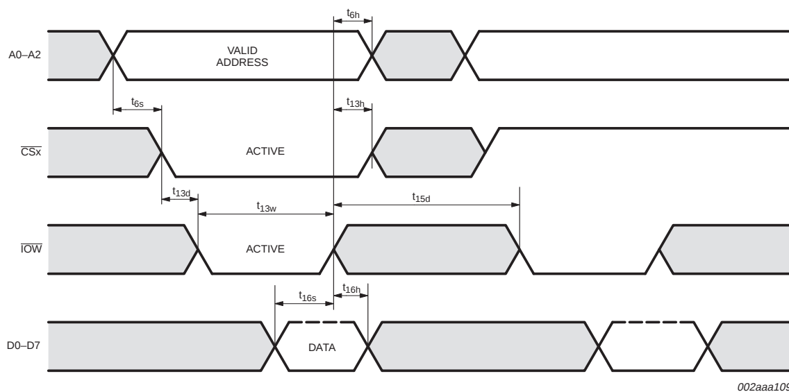
Fig 14. General write timing.
