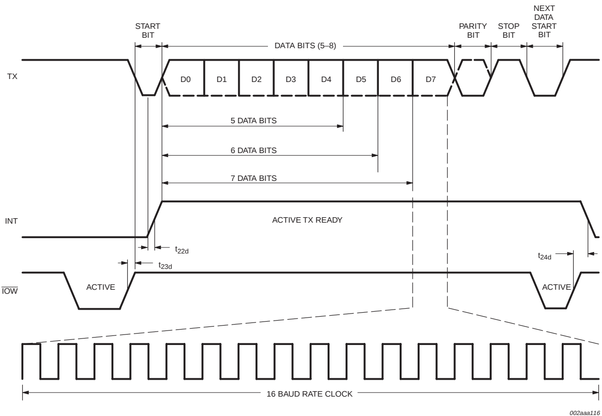
Fig 21. Transmit timing.
