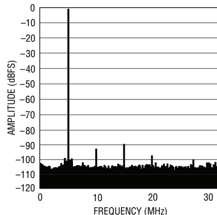
LTC2265-14: 8k Point FFT, f_{IN} = 5\text{MHz} , -1dBFS, 65Mps
