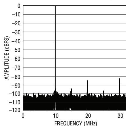
LTC2265-14: 8k Point FFT, f_{IN} = 140\text{MHz} , -1dBFS, 65Mps
