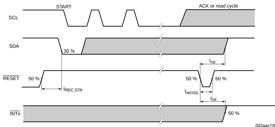
Fig 25. Definition of \overline{\text{RESET}} timing
