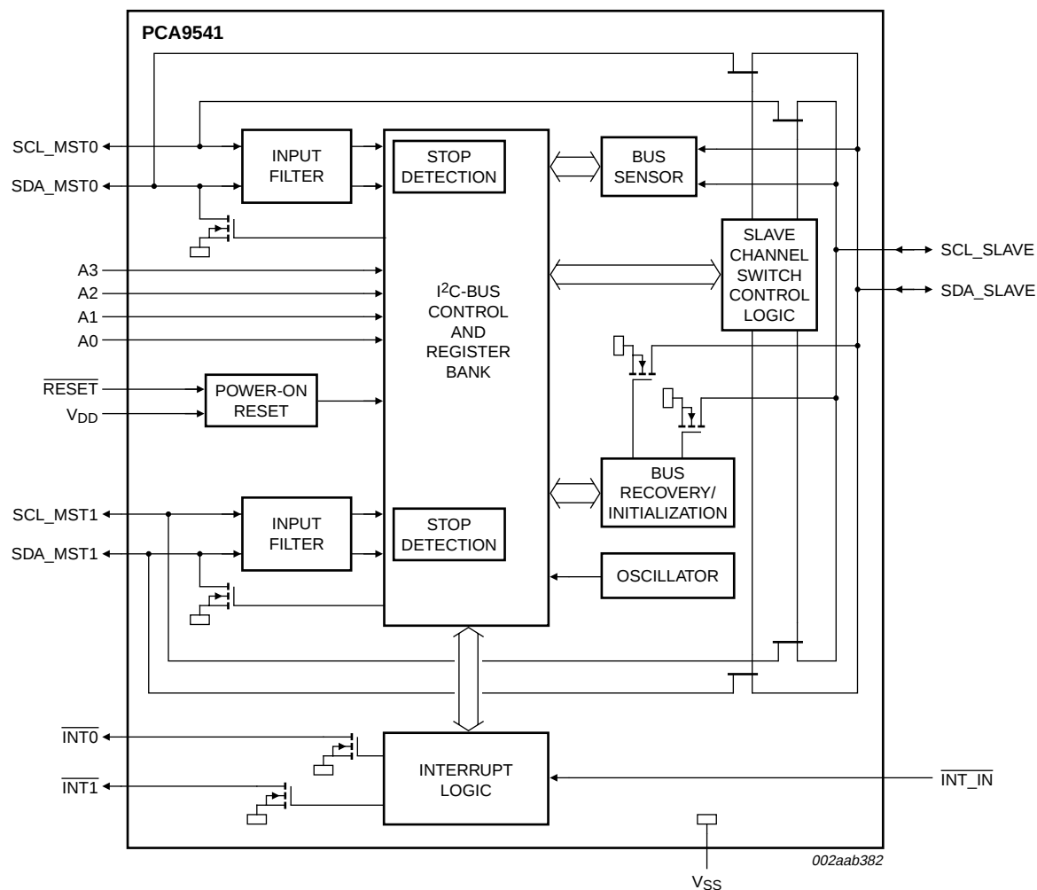
Fig 1. Block diagram of PCA9541
