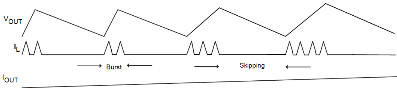
Figure 52. Low Power/Pulse Skipping
