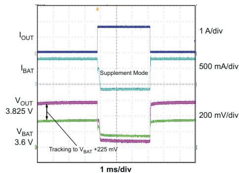
Figure 10-7. Entering and Exiting Battery Supplement Mode BQ24072
