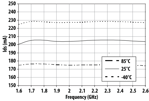
Figure 8. Over Temperature Ids vs Frequency
