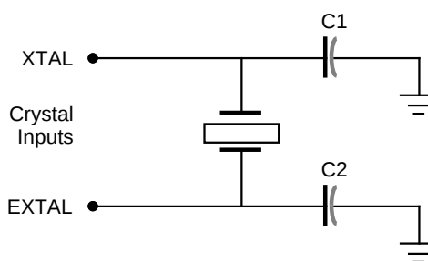
Figure 6. Circuit Configuration For Crystal
