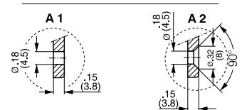
Barbed inserts
