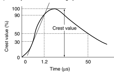
Surge wave form [\pm(1.2 \times 50)\mu s] single polarity full wave voltage
