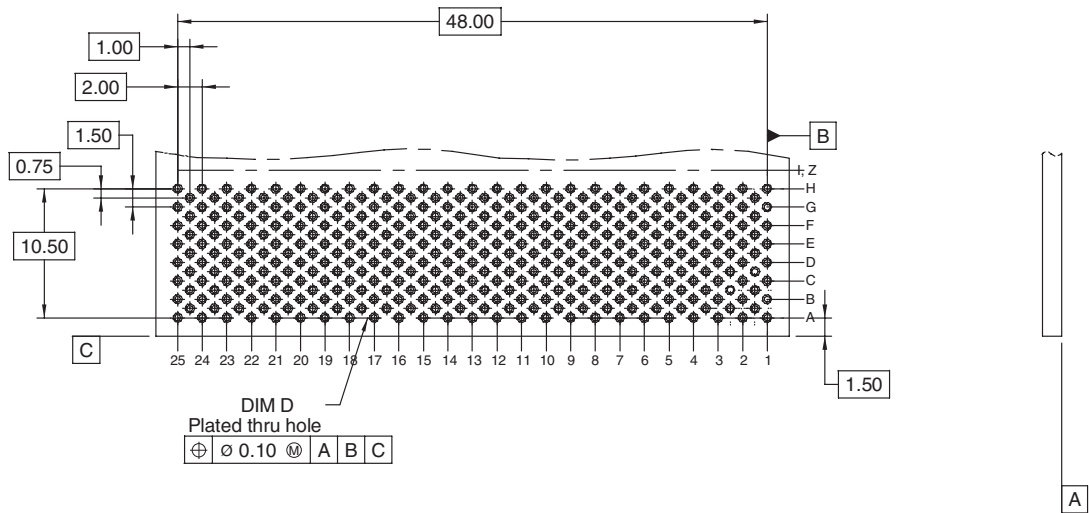
Recommended PCB hole mounting pattern for coaxial, column differential, and stripline applications
