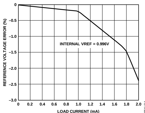
Figure 43. VREF Accuracy vs. Load Current
