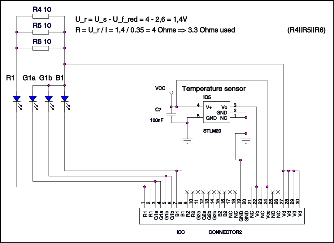
Figure 1. Schematic
