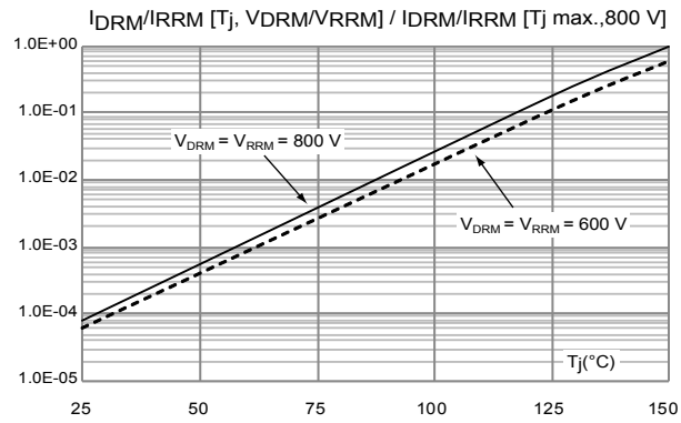
Figure 13. Relative variation of leakage current versus junction temperature for different values of blocking voltage
