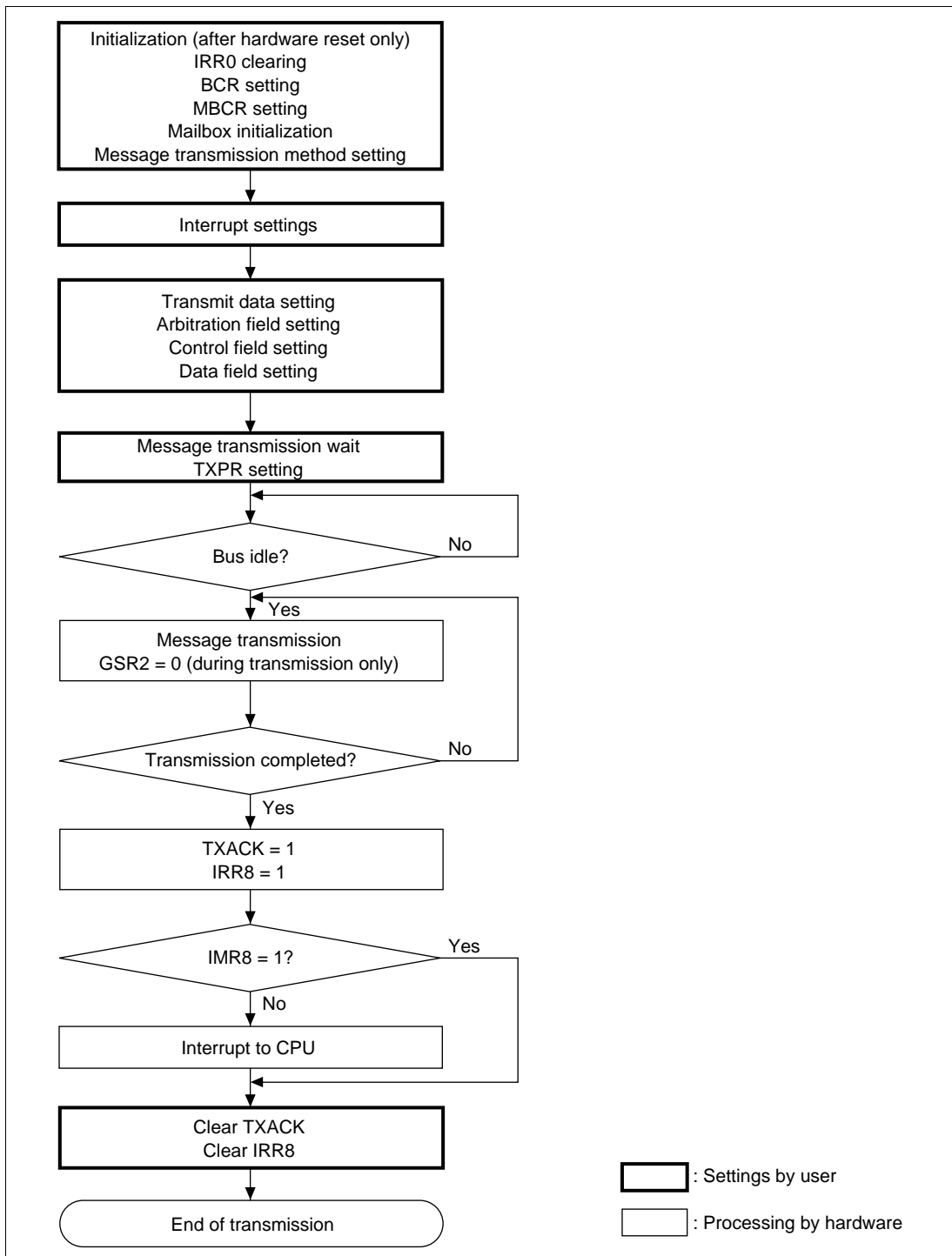
Figure 15-7 Transmission Flowchart
