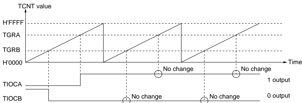
Figure 10-10 Example of 0 Output/1 Output Operation
