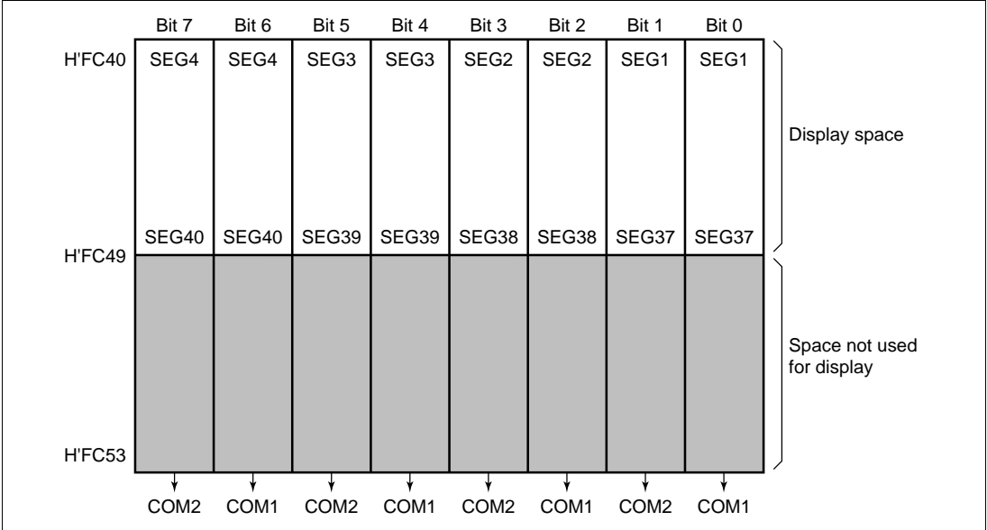
Figure 18-9 LCD RAM Map (1/2 Duty)
