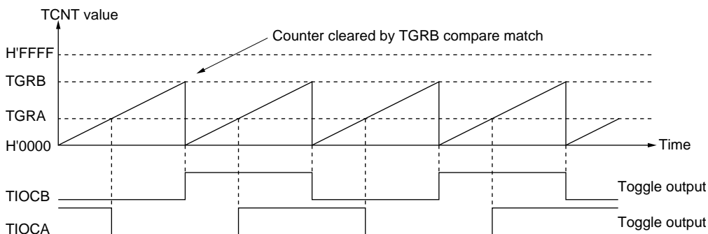
Figure 10-11 Example of Toggle Output Operation
