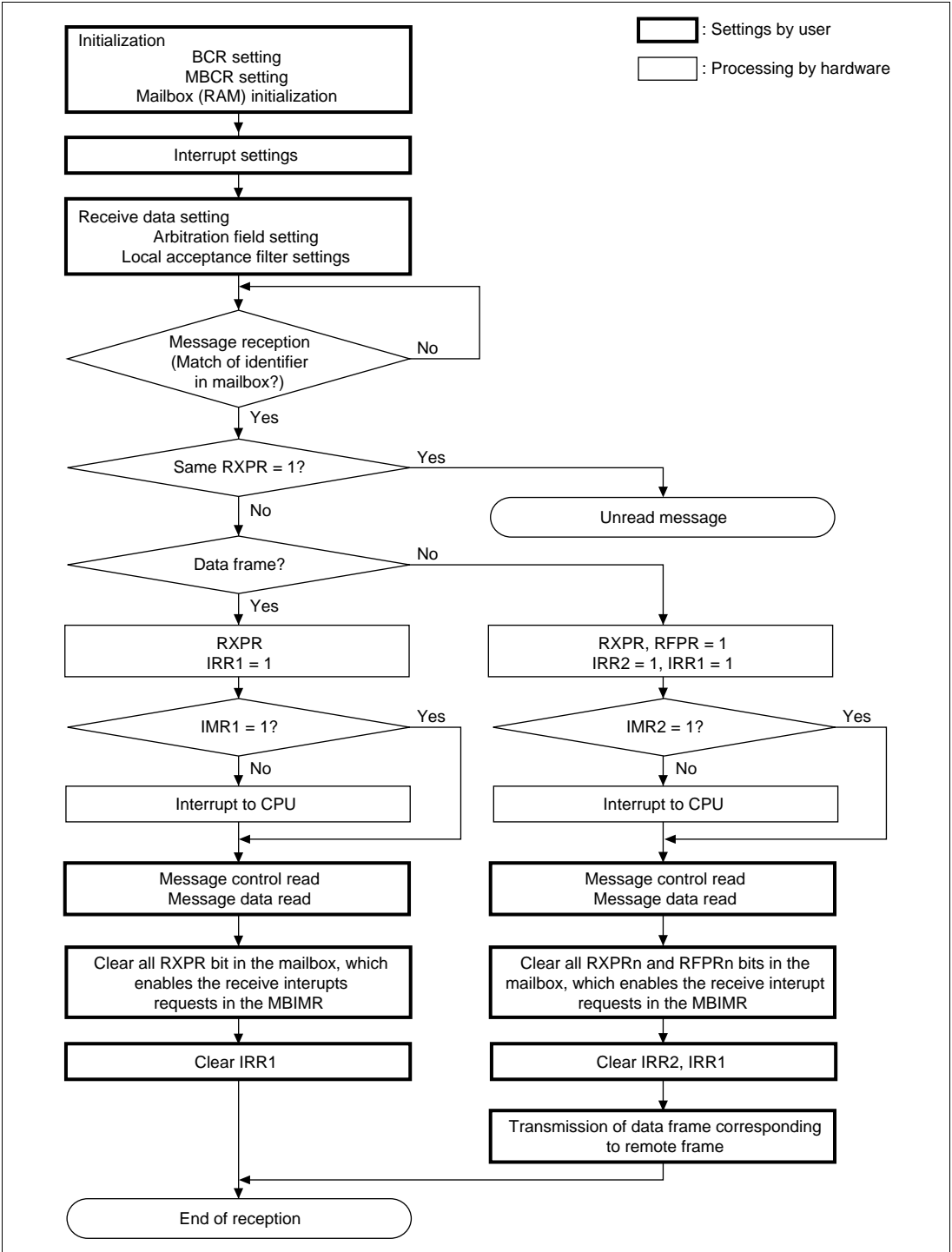
Figure 15-9 Reception Flowchart
