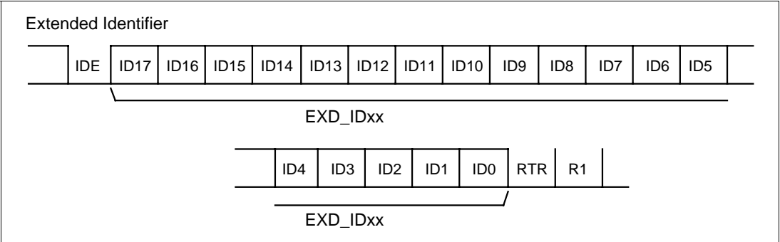
Figure 15-3 Extended Identifier
