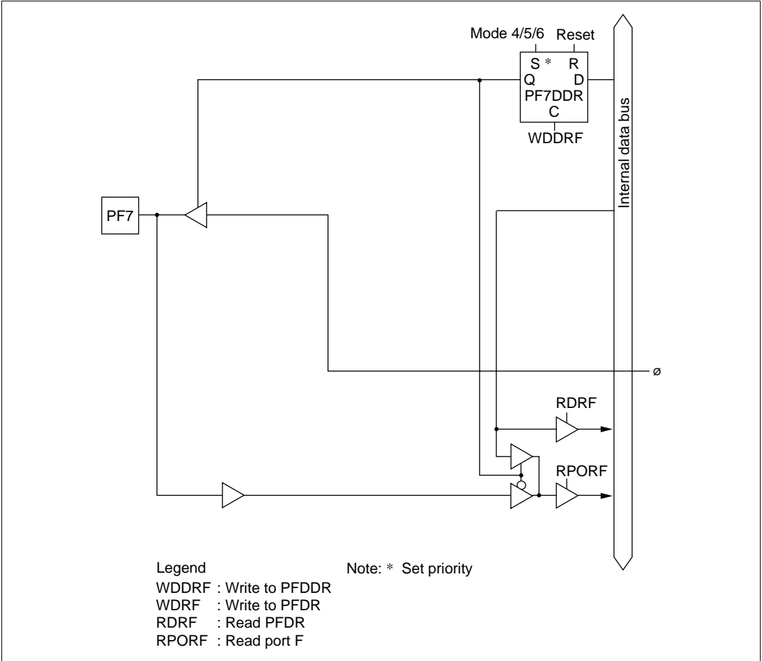
Figure C-12 (g) Port F Block Diagram (Pin PF7)
