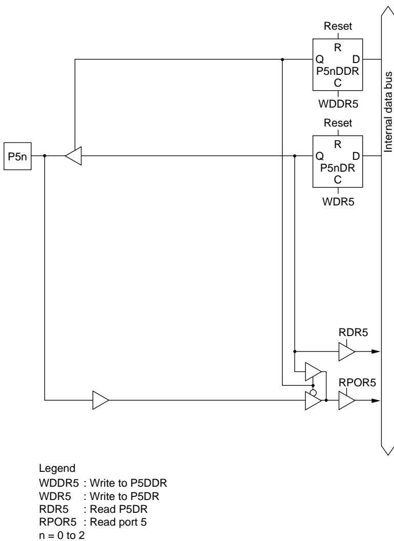
Figure C-5 (a) Port 5 Block Diagram (Pins P50 to P52) (H8S/2646, H8S/2646R, H8S/2645)
