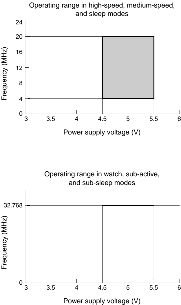
Figure 23-1 Power Supply Voltage and Operating Ranges
