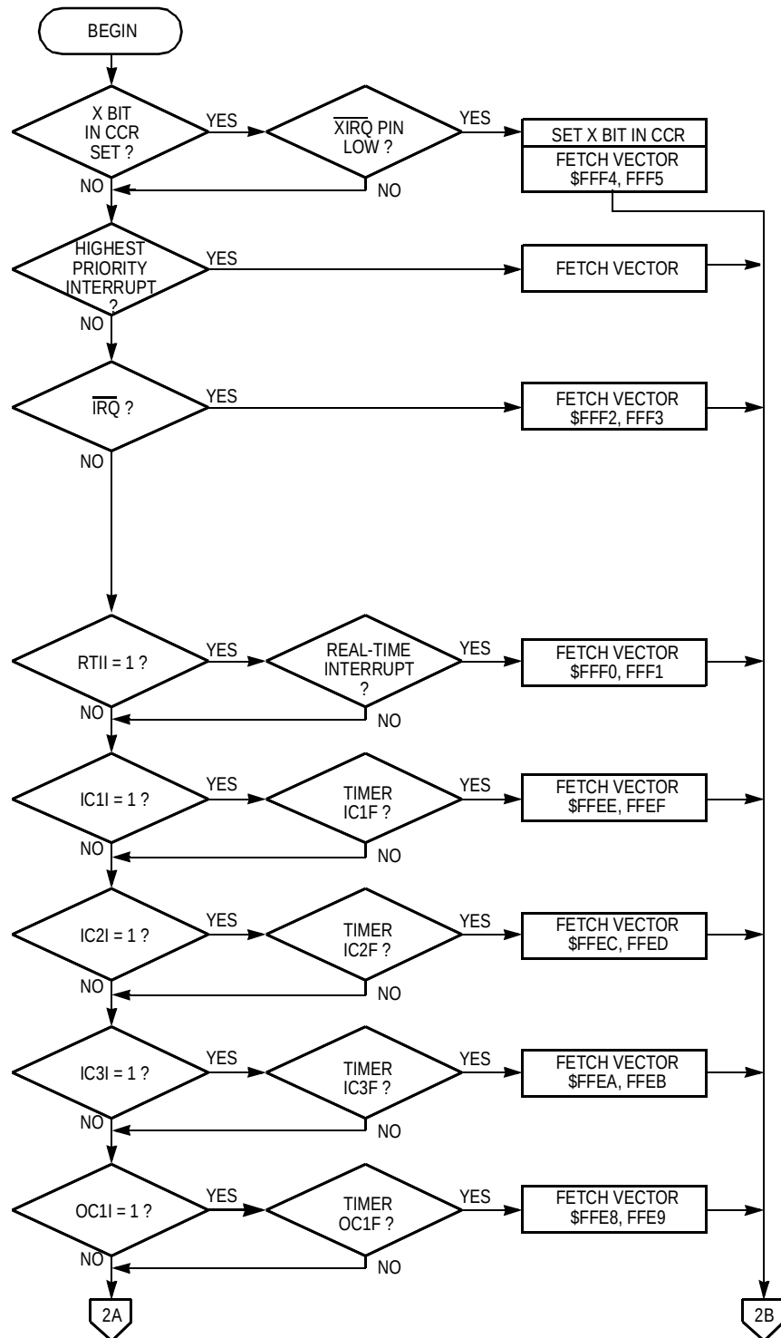
Figure 5-9. Interrupt Priority Resolution (Sheet 1 of 2)
