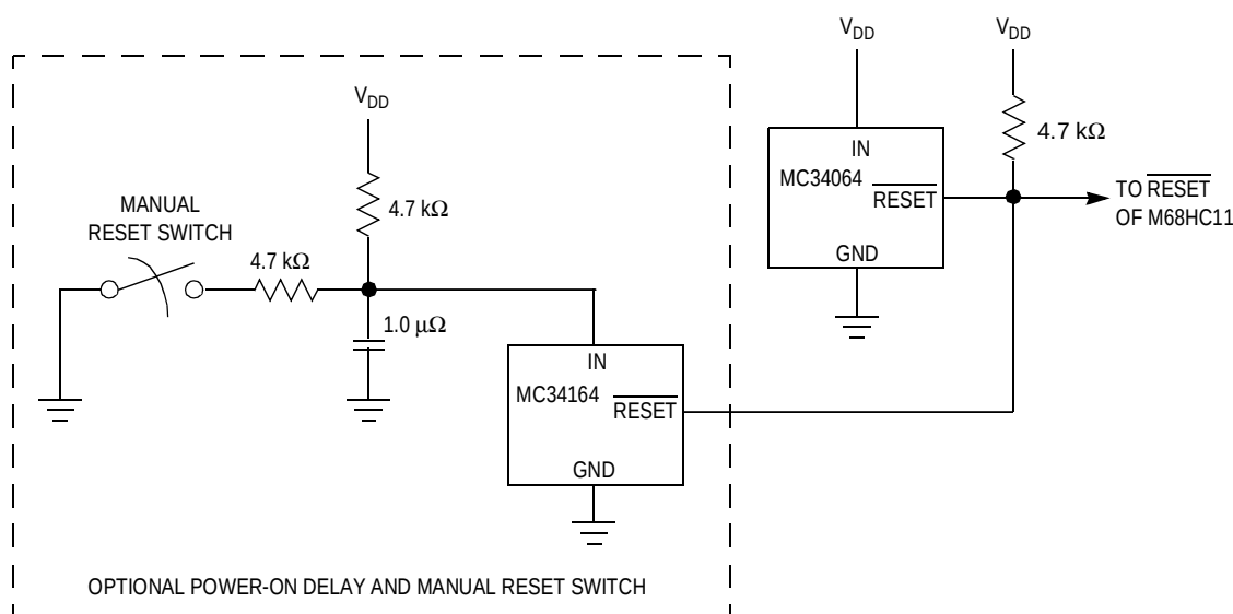
Figure 2-5. External Reset Circuit
