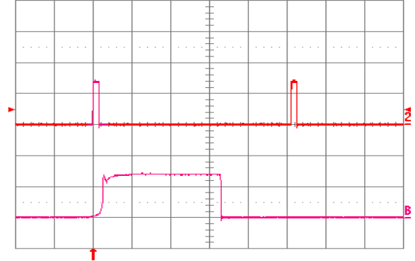
Fig. 1.8V.12: Load current (top trace, 20 A/div., 20 ms/div.) into a 10 mΩ short circuit during restart, at V_{in} = 48 V. Bottom trace (20 A/div., 1 ms/div.) is an expansion of the on-time portion of the top trace.
